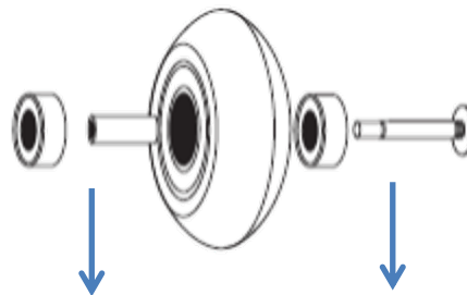
09204200001 BEARING SPACERS ALU 8MM (8PCS)
